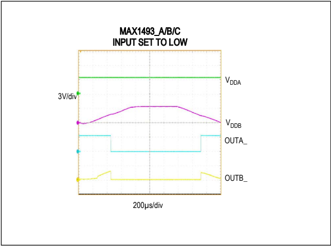
Figure 3. Undervoltage Lockout Behavior (MAX1493_A/BC Low)
