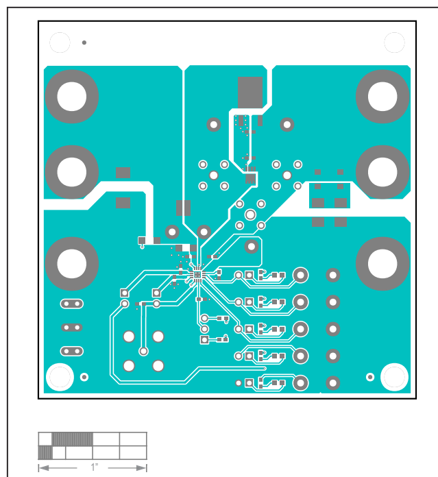
MAX14922 EV Kit PCB Layout—Top View
