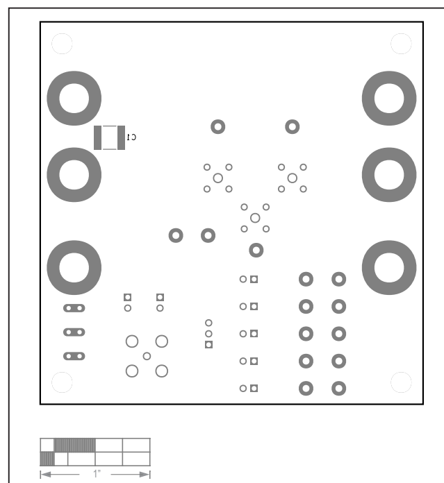
MAX14922 EV Kit PCB Layout—Bottom Silkscreen
