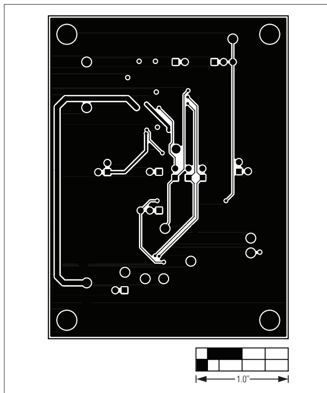
Figure 6. MAX14578A EV Kit PCB Layout—Solder Side
