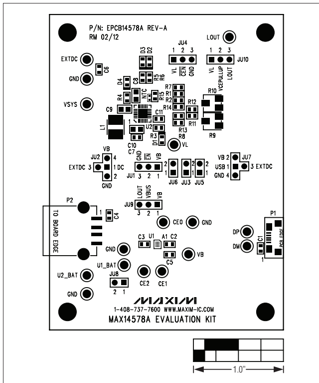
Figure 2. MAX14578A EV Kit Component Placement Guide—Component Side
