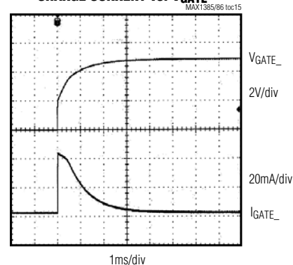
CHARGE CURRENT vs. V GATE
