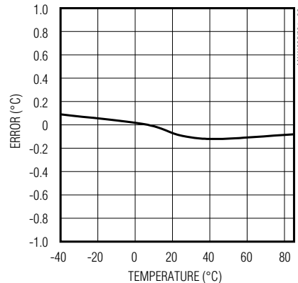
EXTERNAL TEMPERATURE SENSOR ERROR vs. TEMPERATURE
