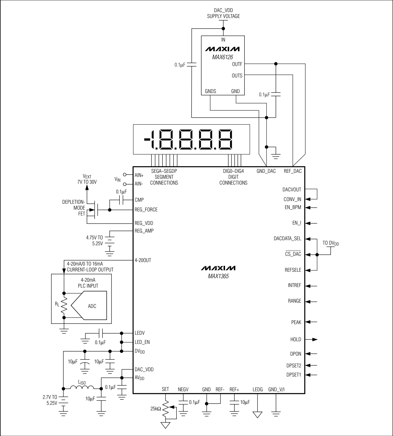
MAX1365 Typical Operating Circuit
