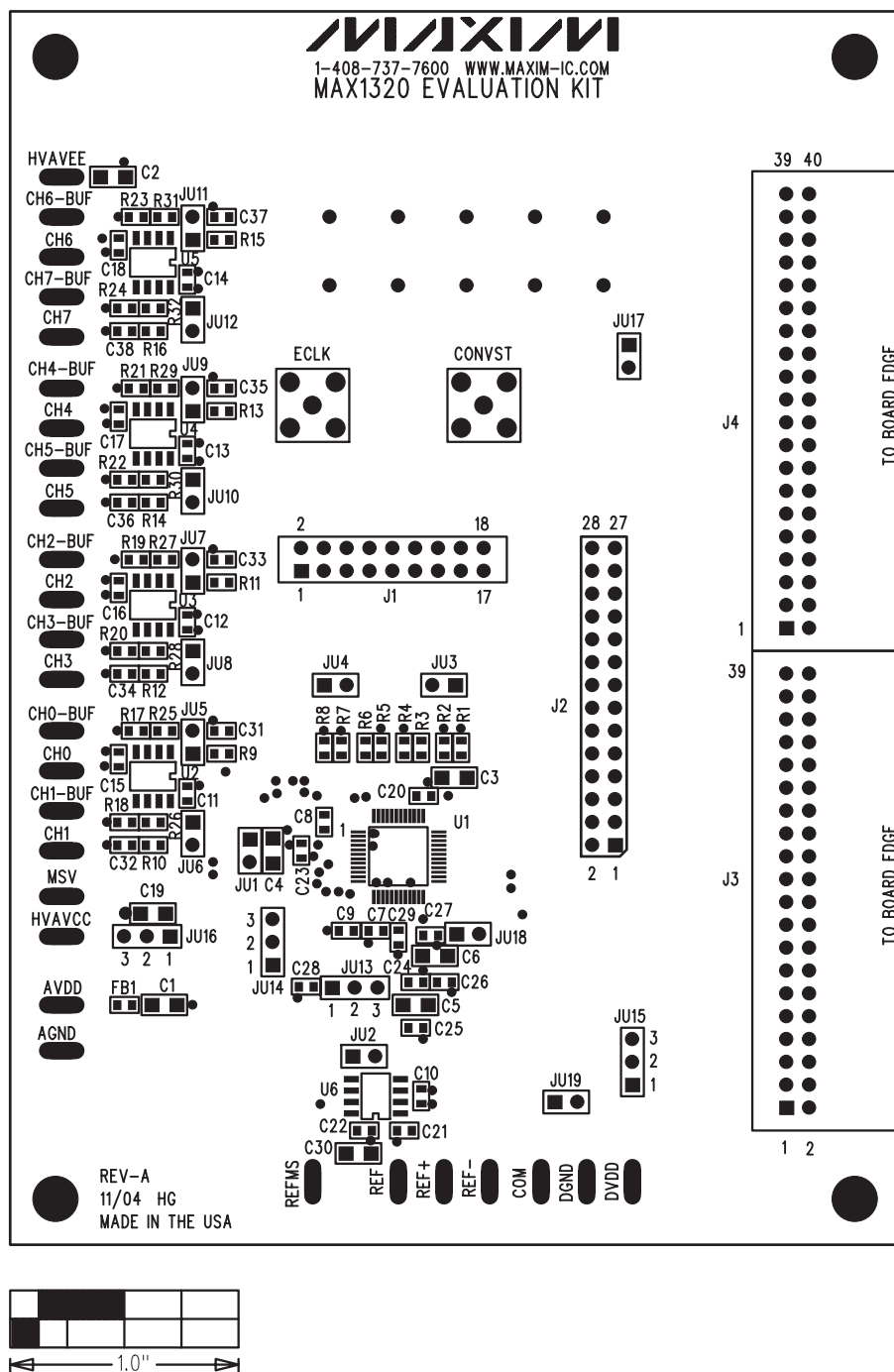
Figure 7. MAX1320 EV Kit Component Placement Guide—Component Side
