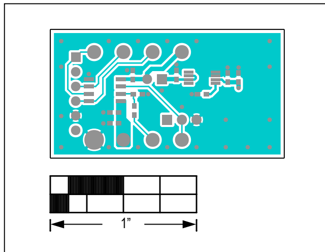
MAX1240 EV Kit—Top
