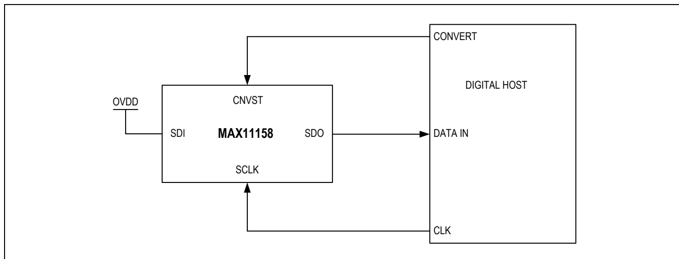
Figure 5. \overline{\text{CS}} Mode 3-Wire, No-Busy Indicator Connection Diagram (SDI High)
