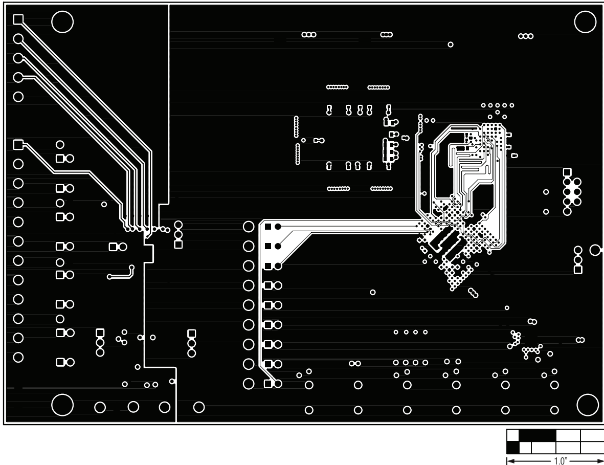
Figure 21. MAX11043 EV Kit PCB Layout—Solder Side
