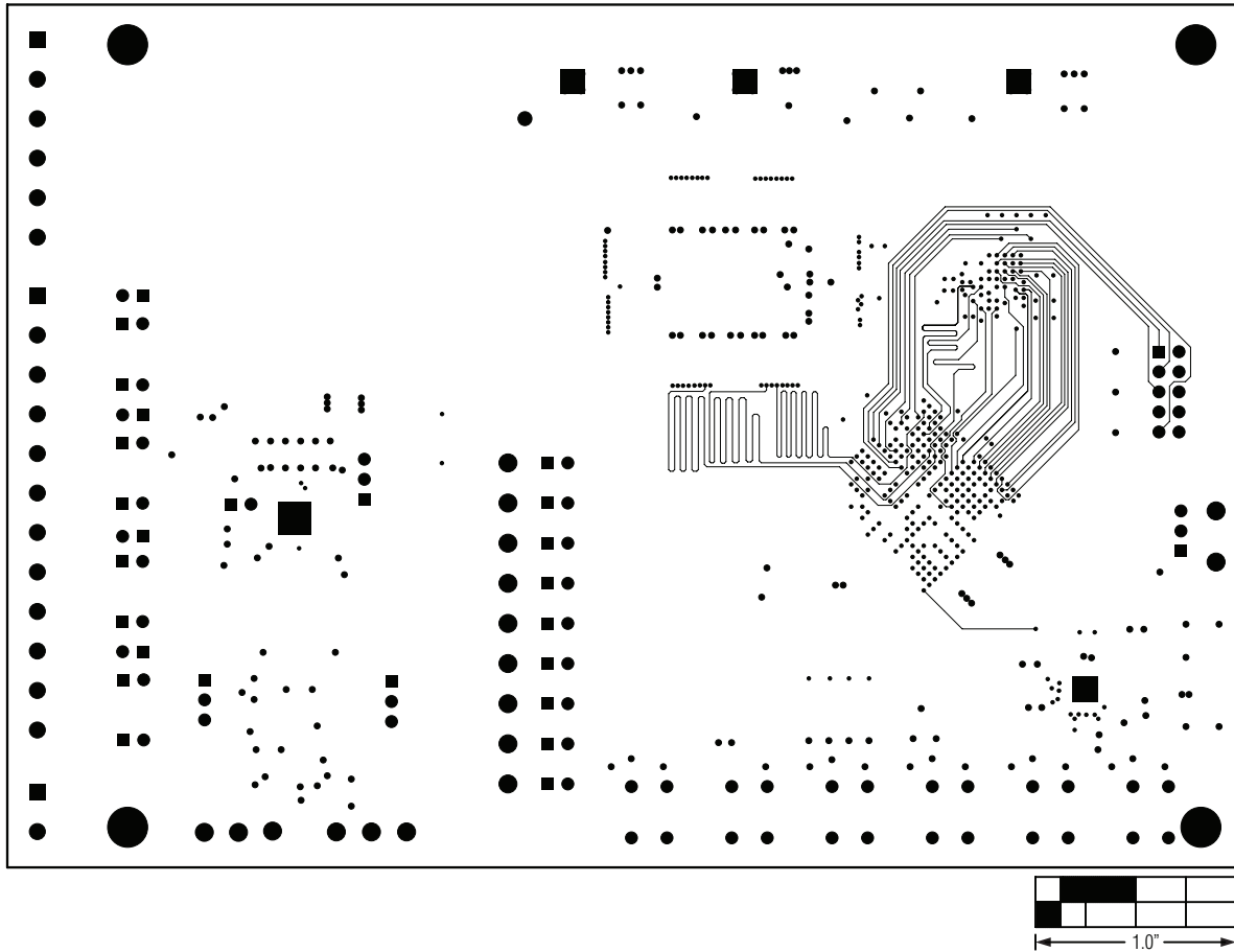
Figure 18. MAX11043 EV Kit PCB Layout—Ground Layer 7
