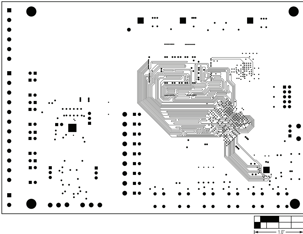
Figure 16. MAX11043 EV Kit PCB Layout—Power Layer 5
