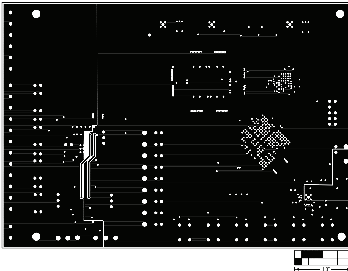
Figure 15. MAX11043 EV Kit PCB Layout—Ground Layer 4
