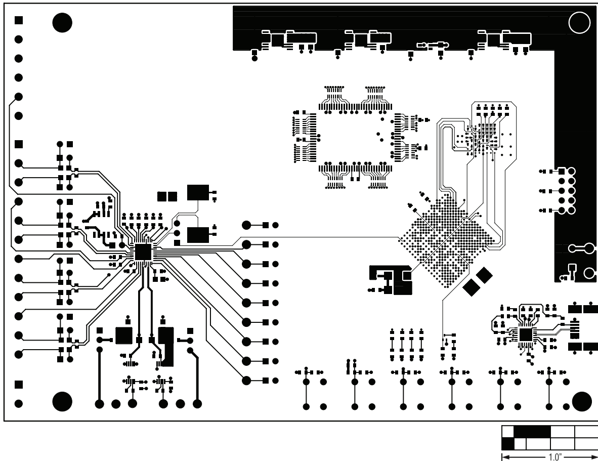
Figure 12. MAX1104311043 EV Kit PCB Layout—Component Side
