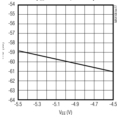
TOTAL HARMONIC DISTORTION vs. V_{EE} ( f_{IN} = 250MHz , -1dB FS)
