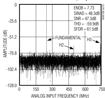
FFT PLOT ( f_{IN} = 1503.021240MHz , -3dB FS, RECORD LENGTH 16,384)
