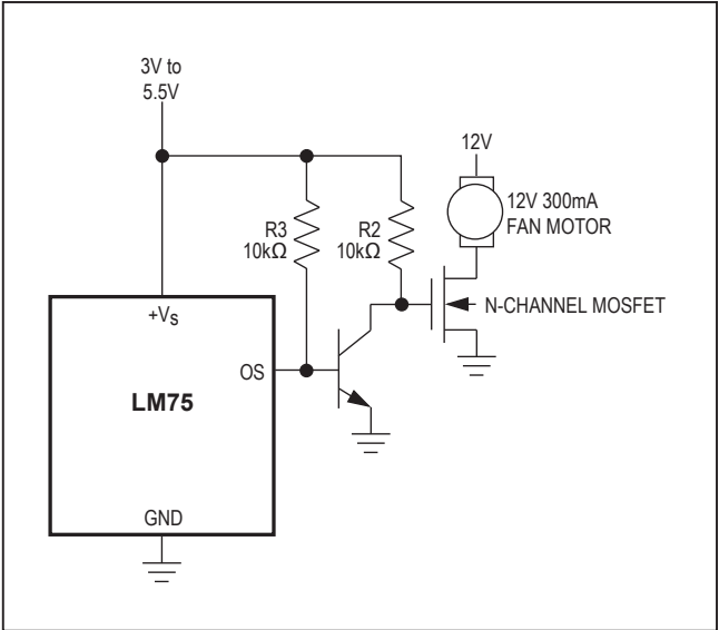
Figure 8. Fan Control
