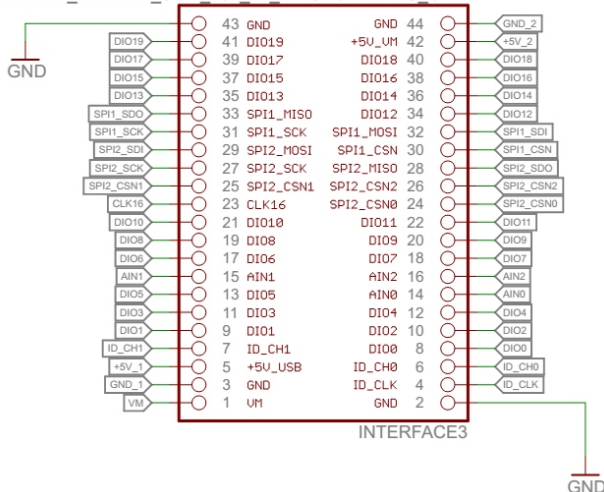
FEMALE_HEADER_SMD 254 44 PINSHORTPADS_ODD
