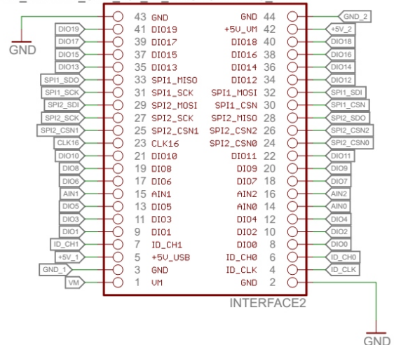
FEMALE_HEADER_SMD 254 44 PINSHORTPADS_EVEN
