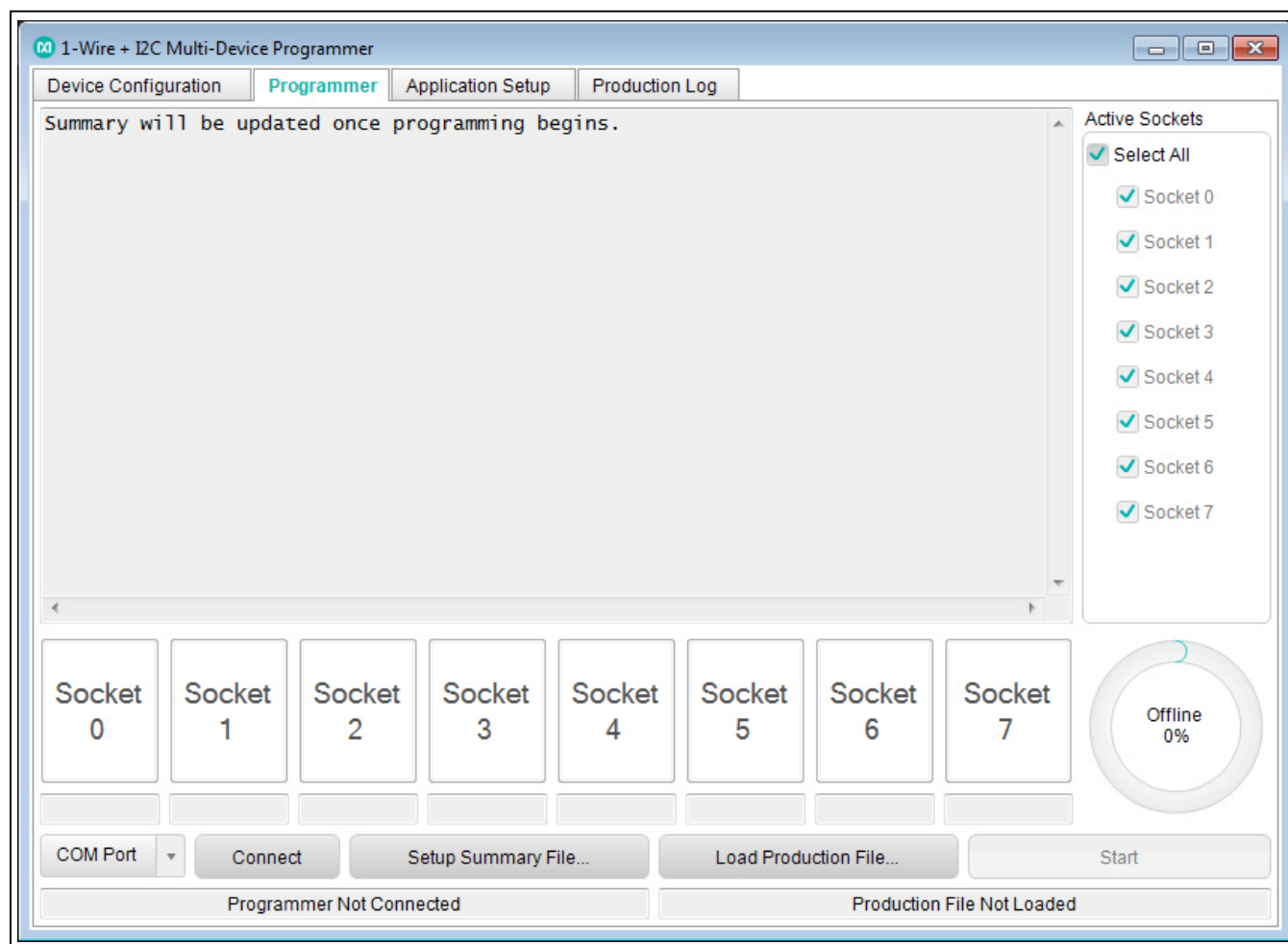
Figure 4. Programming Dialog
