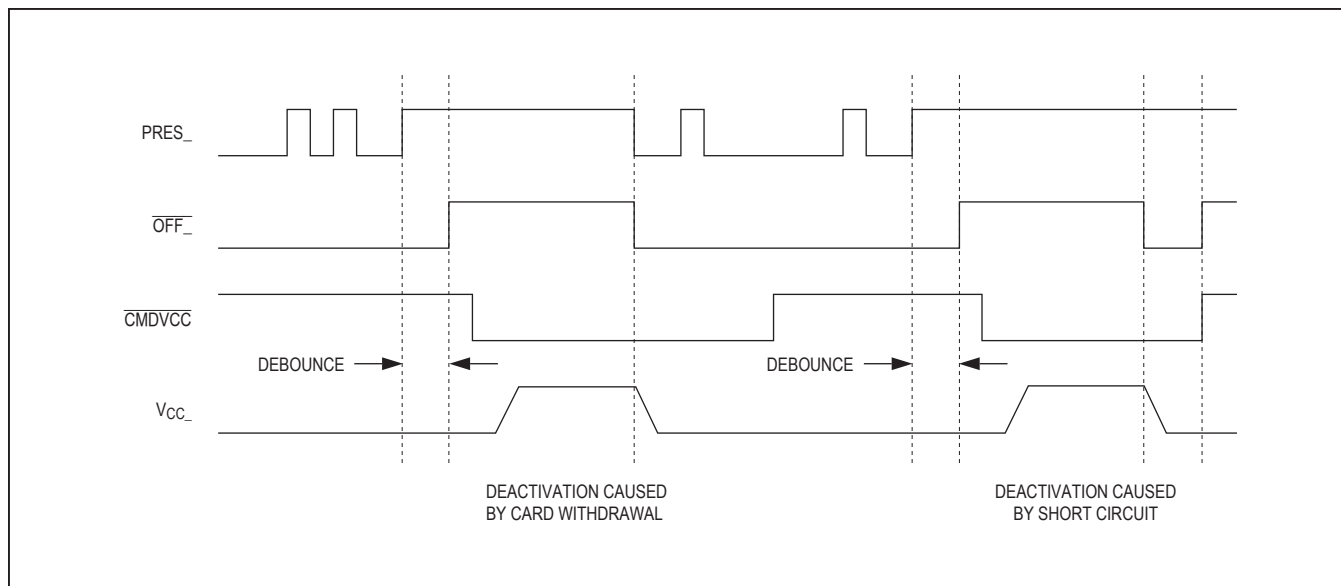
Figure 6. Behavior of PRES_, \overline{\text{OFF\_}} , CMDVCC, and VCC_
