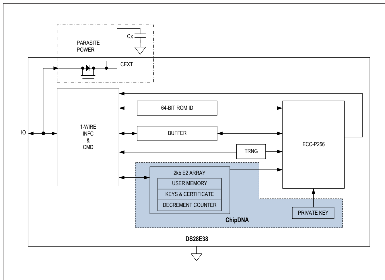
Figure 1. Block Diagram
