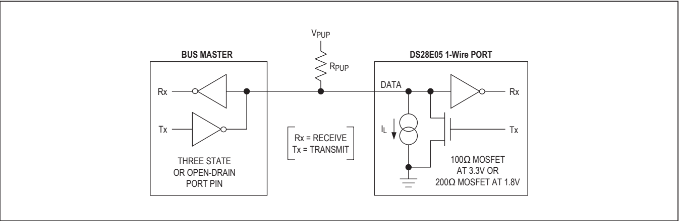
Figure 7. Hardware Configuration
