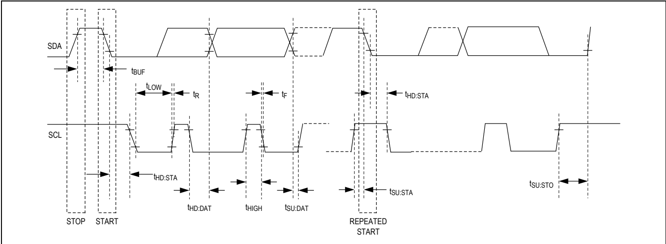
Figure 5. Timing Diagram
