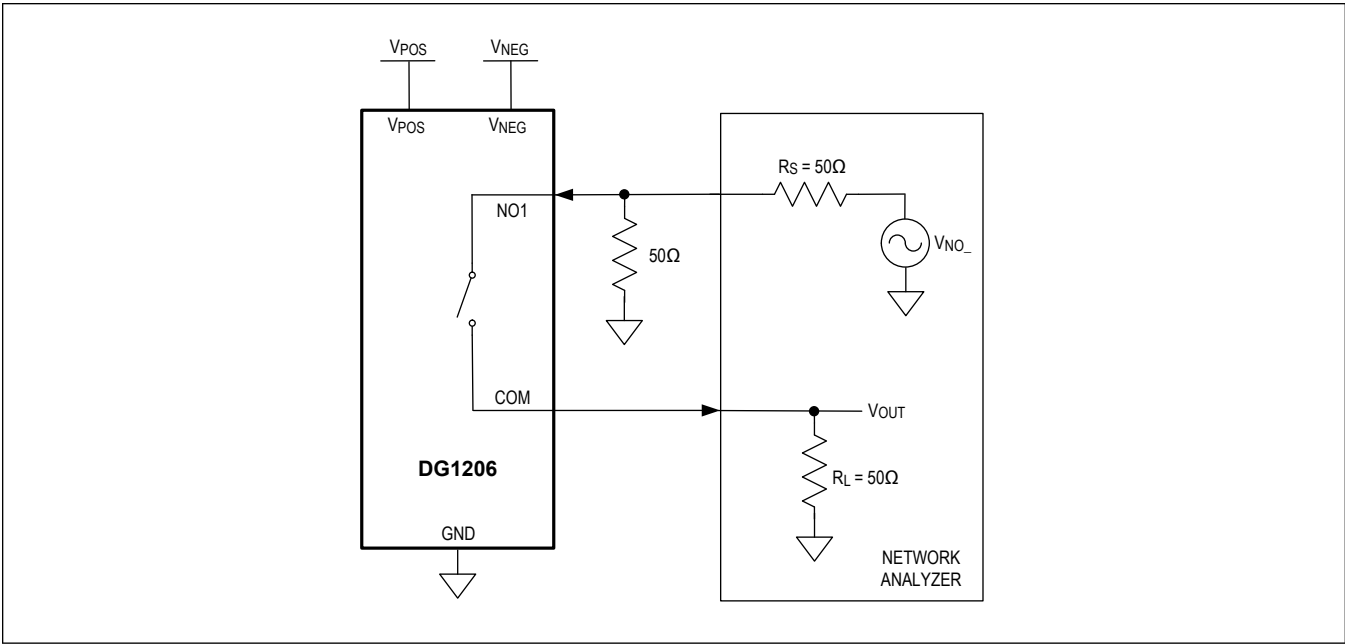
Figure 6. Off-Isolation (Similar Connection for DG1207)
