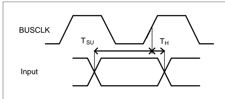
Figure 10: Host Bus Input Timing Diagram
