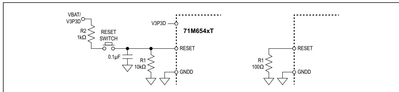
Figure 17. Typical Reset Circuits
