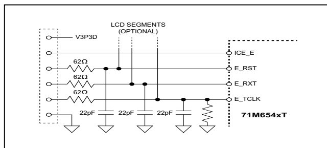
Figure 19. Typical Emulator Connections
