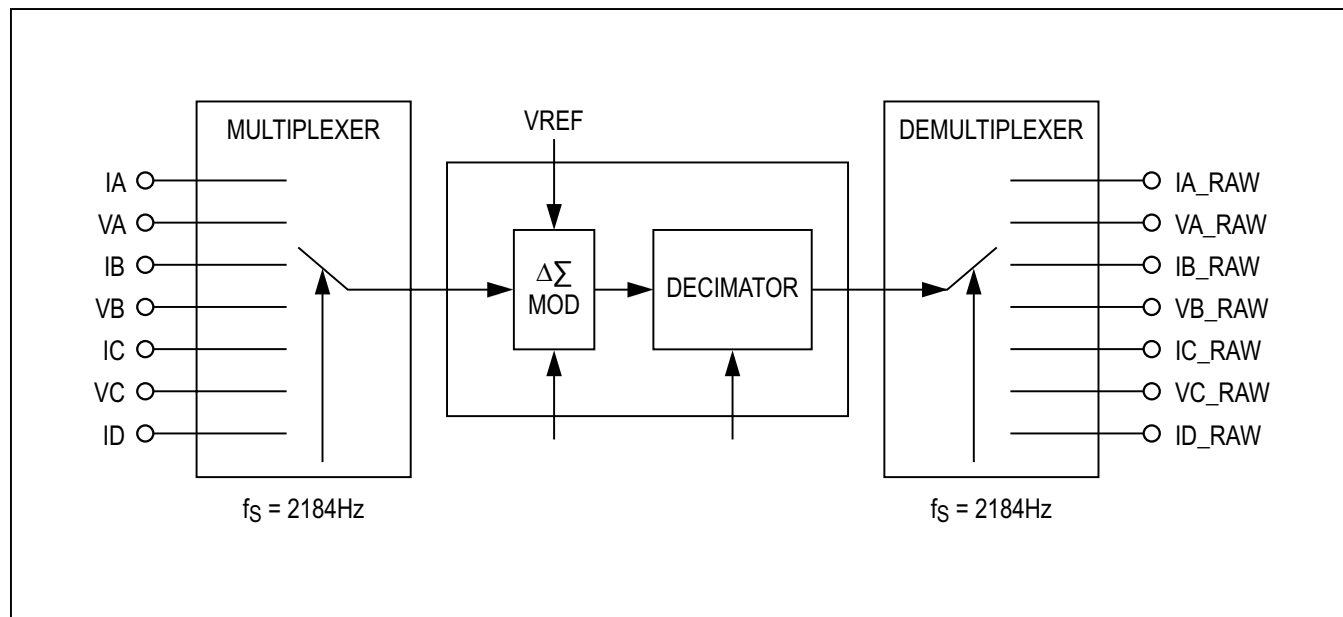
Figure 20. CE Data Flow—Multiplexer and ADC
