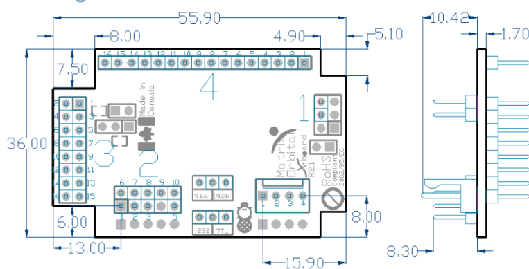
Figure 1: X-Board (S-Series)
