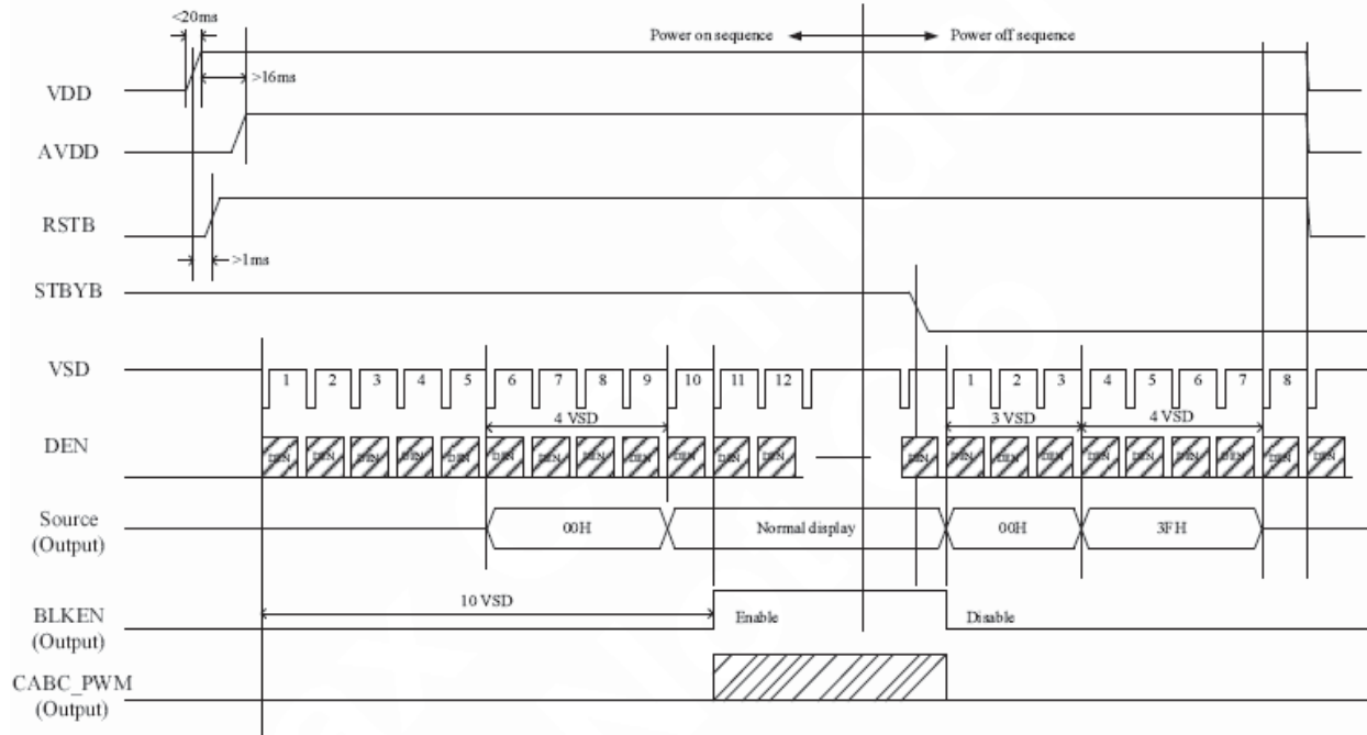
Figure 7: Power up sequence timing diagram
