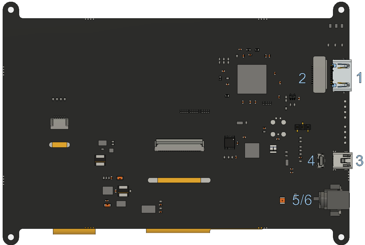
Figure 1: HTT70A Headers
