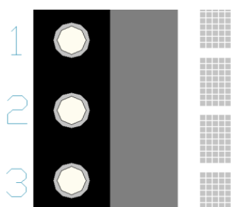
Figure 14: LED Location
