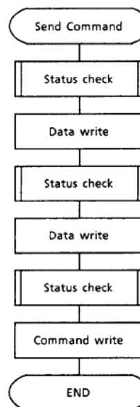
Figure 3: Two Byte Command
