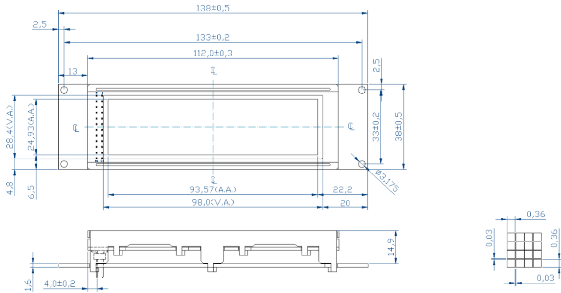
Figure 1: MOP-GL24064A Mechanical Drawing
