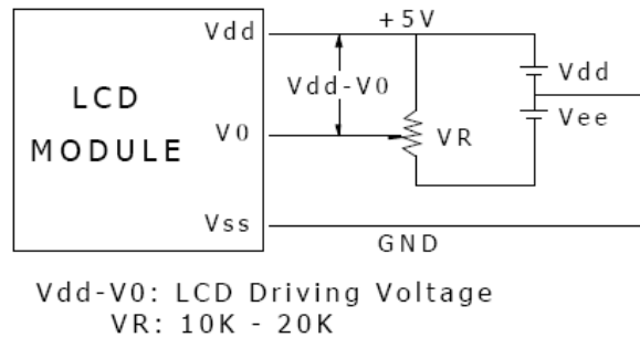
Figure 8: Dual Supply Configuration
