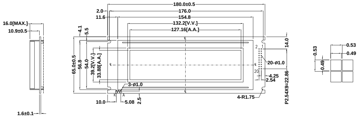
Figure 1: MOP-GL24064A Mechanical Drawing
