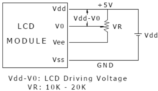
Figure 7: Single Supply Configuration
