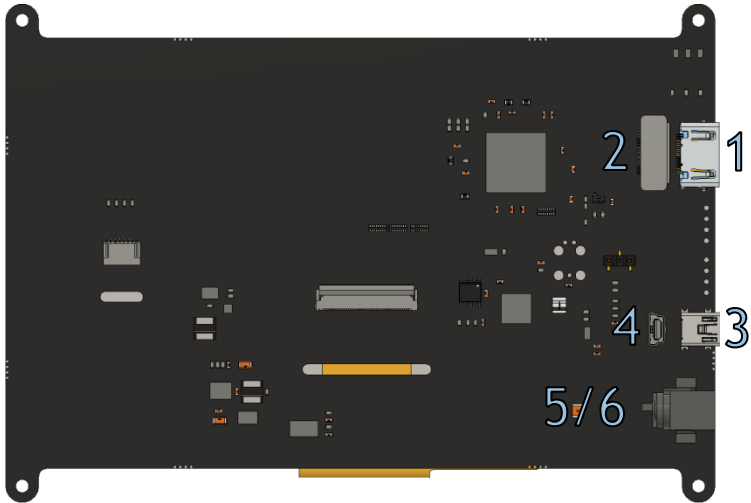
Figure 2: HTT70A Headers
