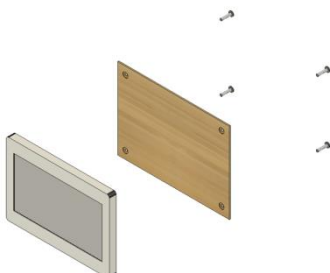
Figure 17: Display Assembly Installation
