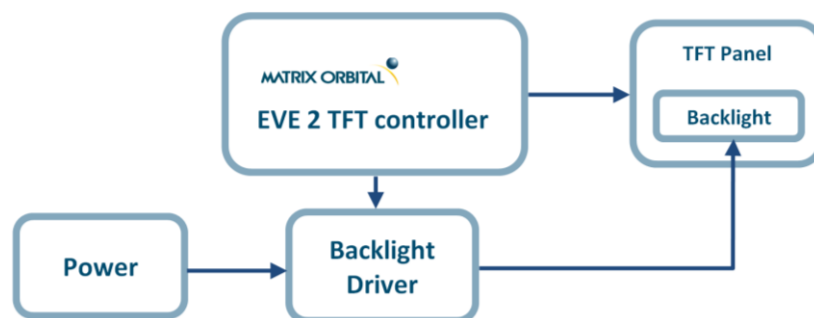
Figure 12: Backlight Driver Block Diagram
