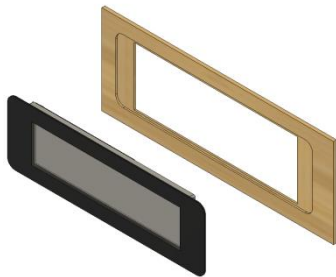
Figure 13: EVE2-38G Installation
