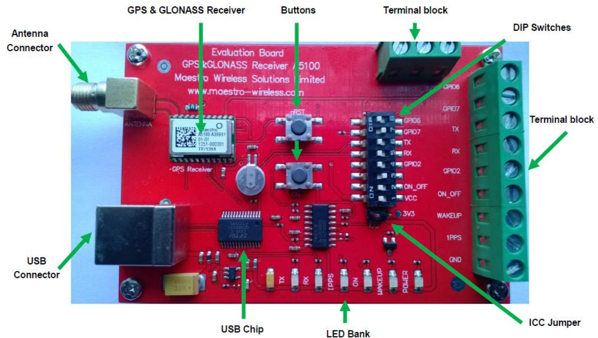
Figure 9: Board overview
