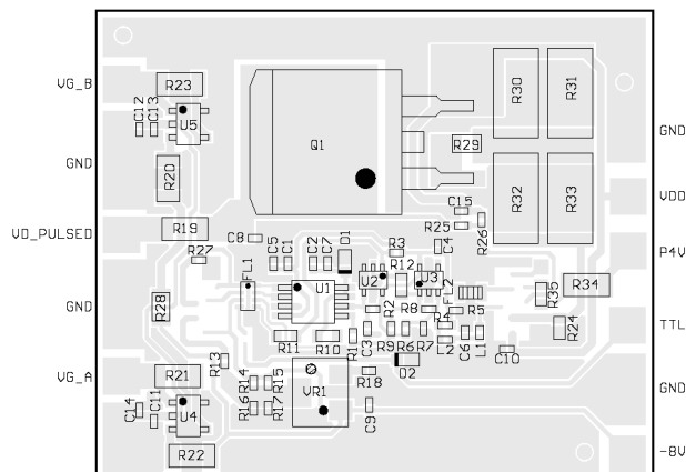
Figure 3. Populated MABC-001000-PB2PPR Evaluation Board
