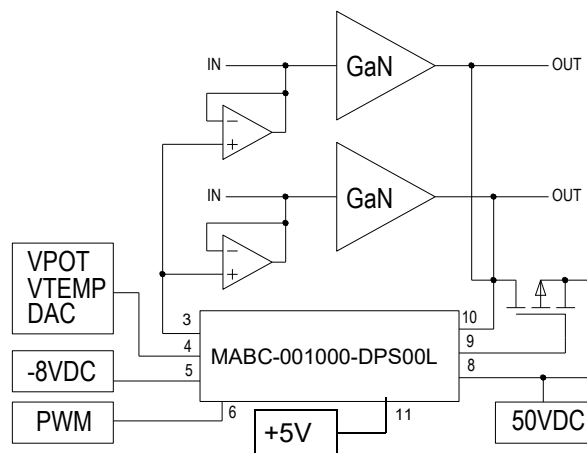
Figure 4. MABC-001000-PB2PPR with MABC-001000-DPS00L Mounted
