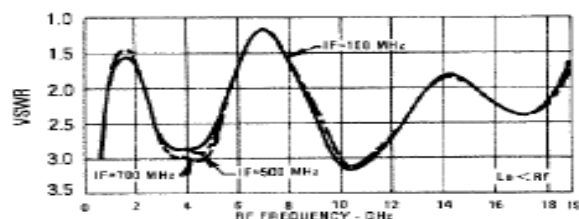
R-Port VSWR vs. Frequency
