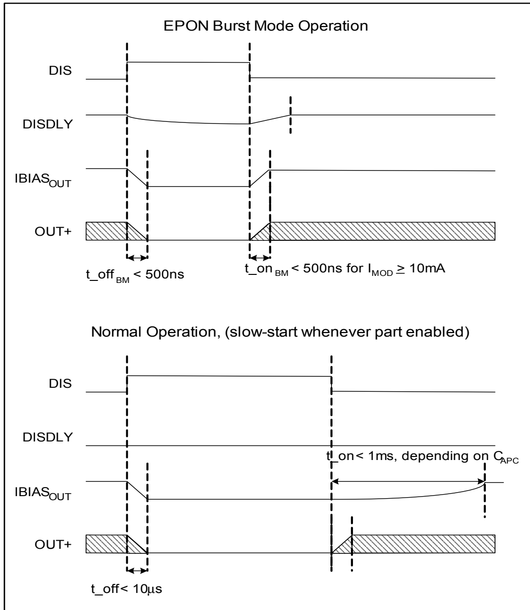
Figure 3-7. DIS and DISDLY Timing
