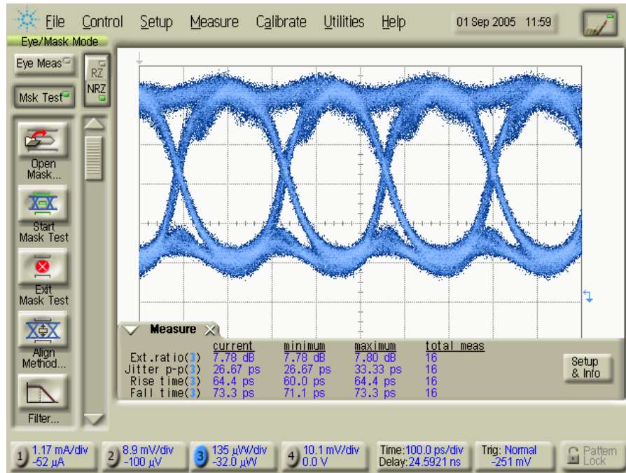
Figure 3-4. 4.25Gbps Unfiltered Optical Eye Diagram with Archcom AC3460 Laser
