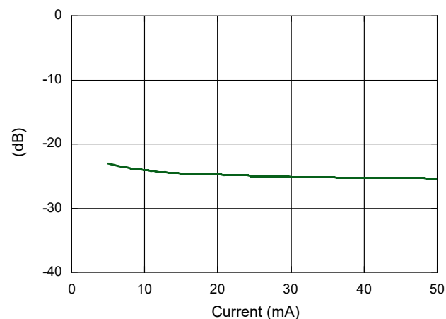
Output Return Loss vs. Bias Current
