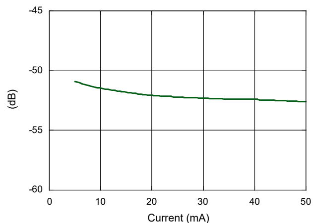
Isolation vs. Bias Current
