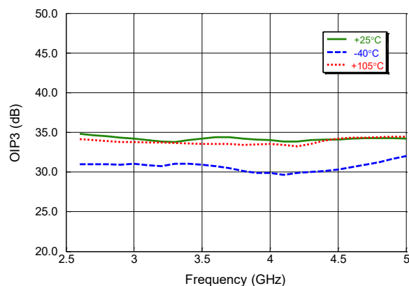
Channel 1 OIP3 over swept Frequency (& Temp.) with P_{OUT}/\text{Tone} = 3 dBm & 10 MHz tone spacing in HGM.
