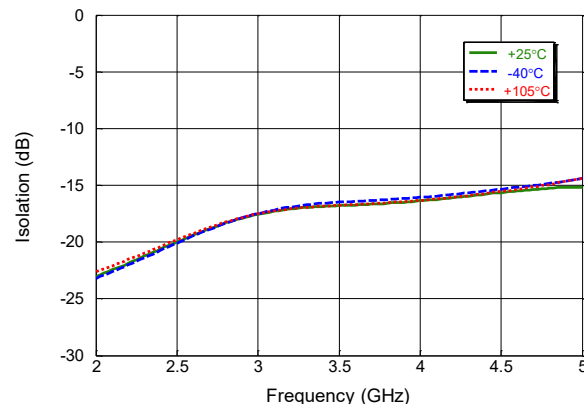
Channel 2 ANT to LOAD Isolation over swept Frequency (& Temp.) in Rx Low Gain Mode
