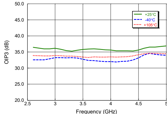
Channel 2 OIP3 over swept Frequency (& Temp.) with P_{OUT}/\text{Tone} = 3 dBm & 10 MHz tone spacing in HGM.
