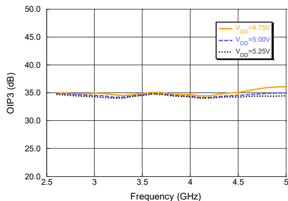
Channel 1 OIP3 over swept frequency (& V_{DD} ) with P_{OUT}/\text{Tone} = 10 dBm & 10 MHz tone spacing in HGM.
