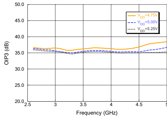
Channel 2 OIP3 over swept frequency (& V_{DD} ) with P_{OUT}/\text{Tone} = 10 dBm & 10 MHz tone spacing in HGM.
