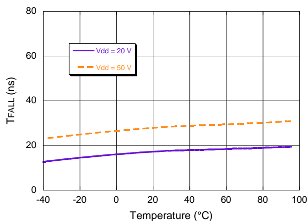
Switching Speed Driving 100 pF Capacitors: T_{FALL}
