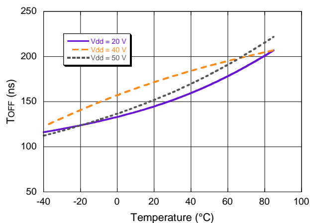
Switching Speed Driving MASW-000936: R_x OFF
