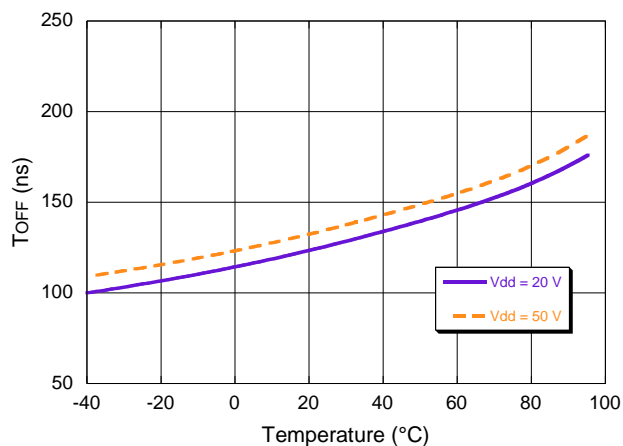
Switching Speed Driving 100 pF Capacitors: T_{OFF}
