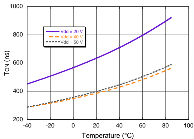
Switching Speed Driving MASW-000936: R_x ON
