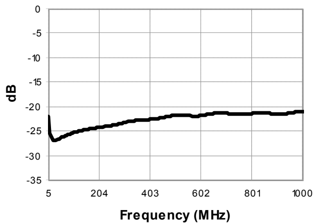
Return Loss Coupling (pin 4)
