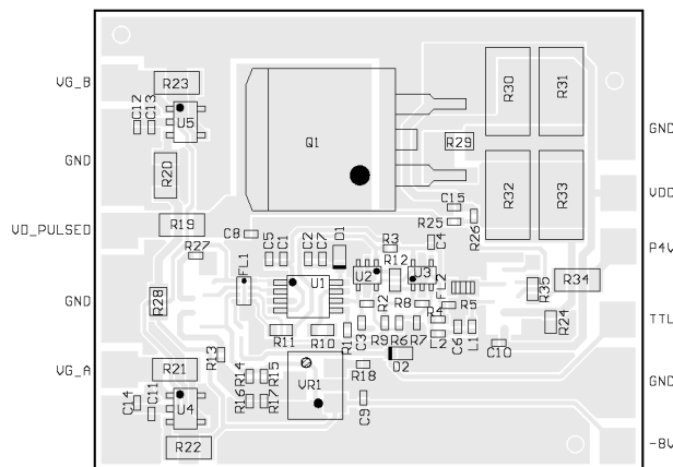
Figure 3. Populated MABC-001000-PB1PPR Evaluation Board
