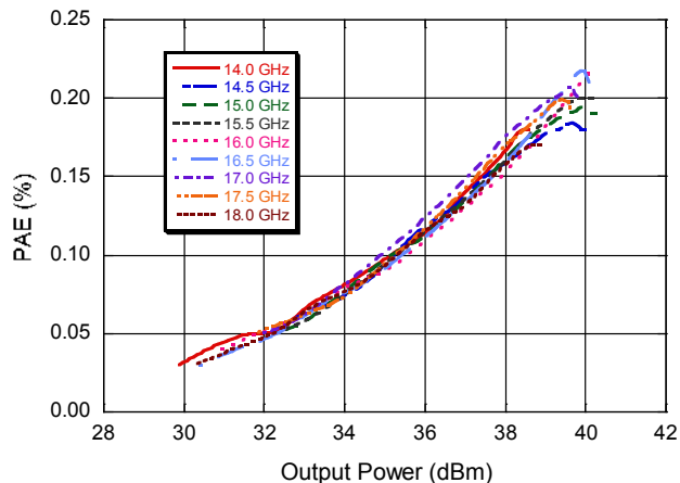
PAE vs. Output Power
