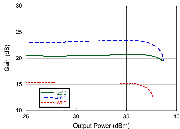
Gain @ 15.5 GHz vs. Output Power
