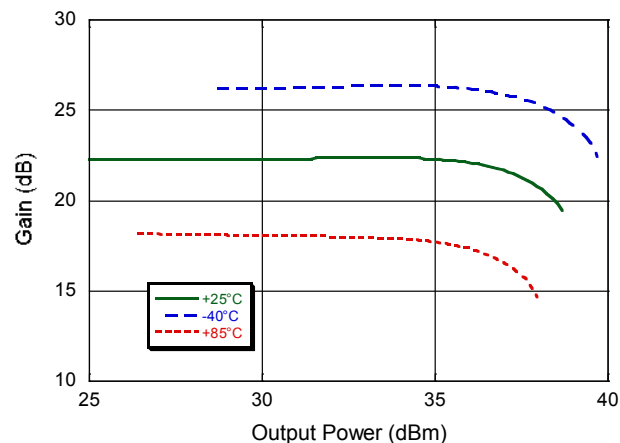
Gain @ 14.5 GHz vs. Output Power
