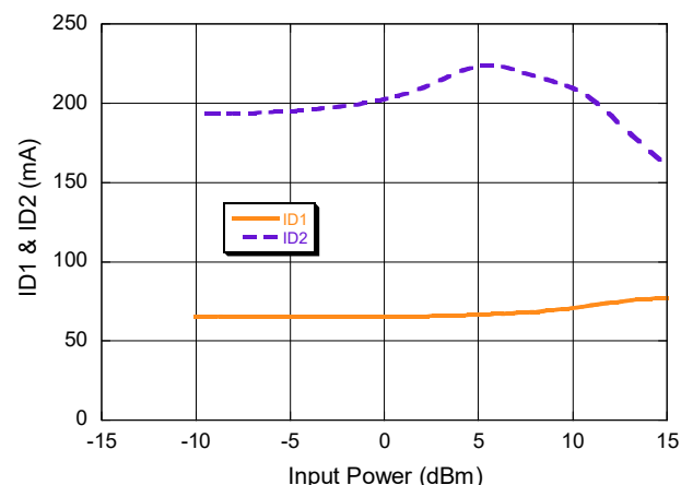
Bias Current vs. P_{IN} @ 2.5 GHz
