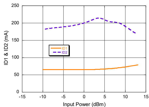
Bias Current vs. P_{IN} @ 1600 MHz
