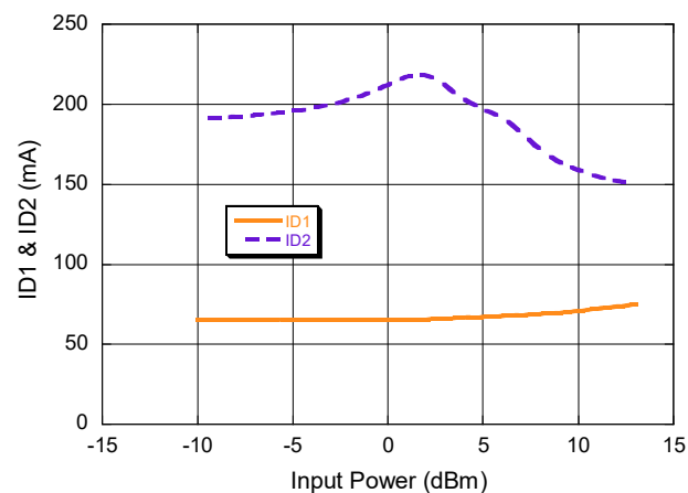
Bias Current vs. P_{IN} @ 1100 MHz
