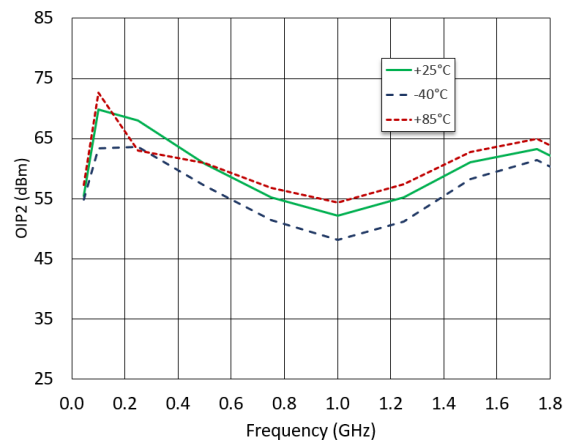
OIP2, P_{OUT} = +5\text{ dBm/tone}
