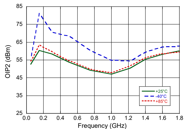
OIP2, P_{OUT} = +5\text{ dBm/tone}
