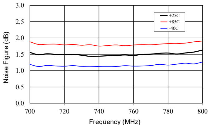
Noise Figure
