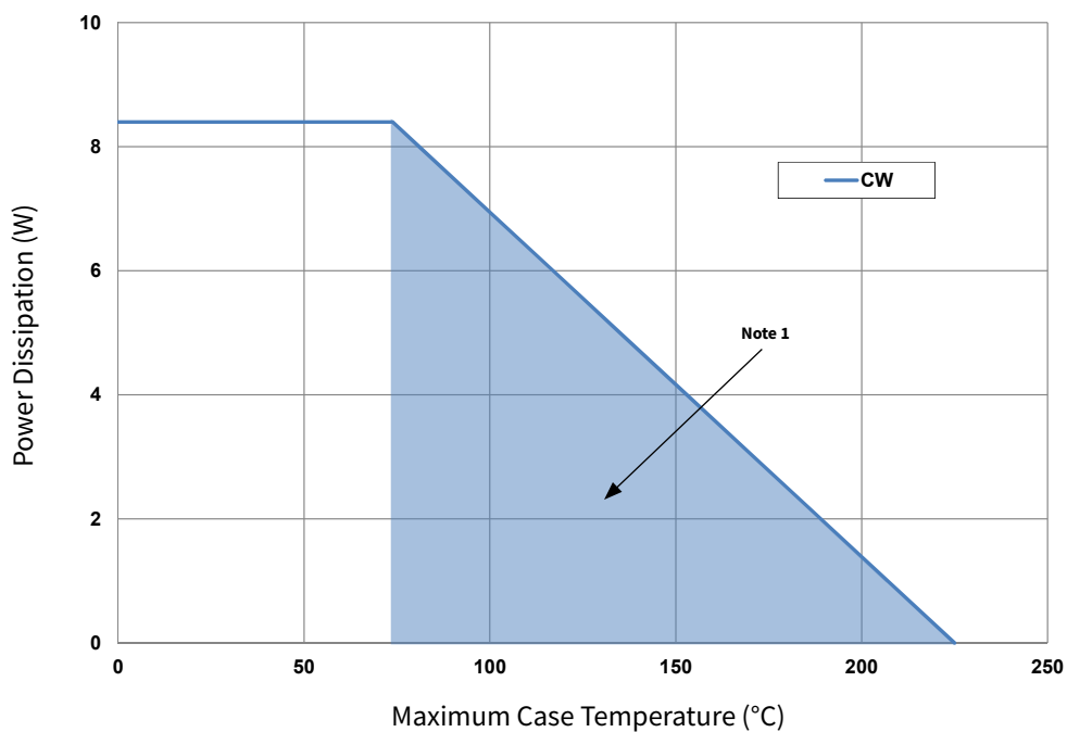
Figure 6. Transient Power Dissipation De-Rating Curve
