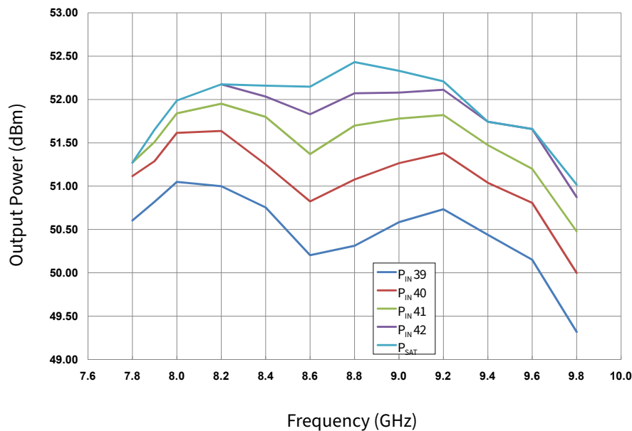
Figure 7. Output Power vs Input Power & Frequency V_{DD} = 40 V, Pulse Width = 100μsec, Duty Cycle = 10%
