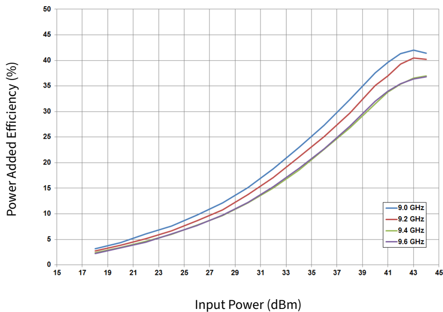
Figure 5. Power Added Efficiency vs Input Power V_{DD} = 40 V, Pulse Width = 100 \mu sec, Duty Cycle = 10%
