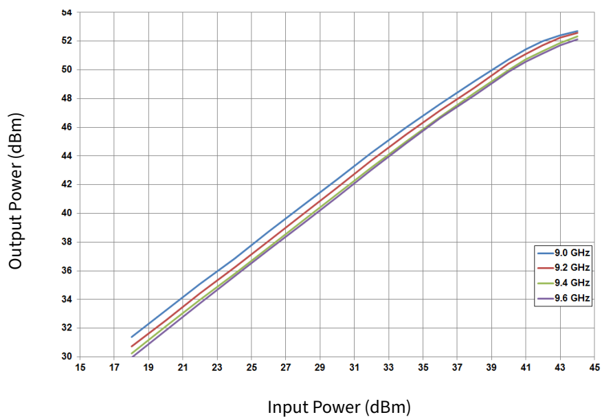
Figure 3. Output Power vs Input Power V_{DD} = 40 V, Pulse Width = 100 \mu sec, Duty Cycle = 10%
