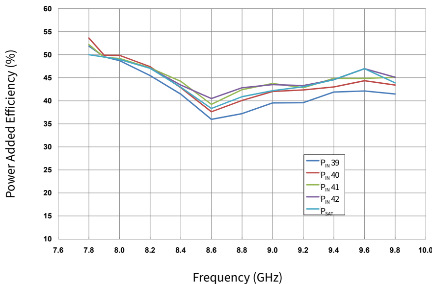
Figure 8. Power Added Efficiency vs Input Power & Frequency V_{DD} = 40 V, Pulse Width = 100μsec, Duty Cycle = 10%
