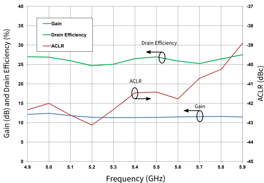
Figure 12. Typical Gain, Efficiency and WCDMA Performance vs Frequency
