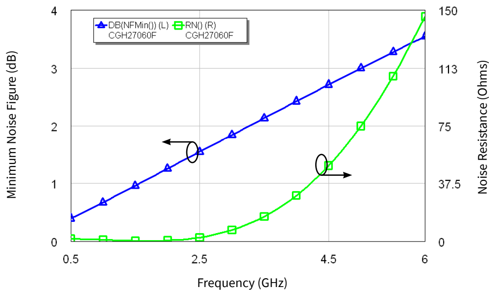
Figure 6. Simulated Minimum Noise Figure and Noise Resistance vs Frequency of the CGH27060F V_{DD} = 28\text{ V} , I_{DQ} = 100\text{ mA}
