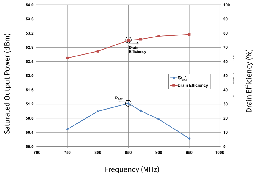
Figure 2. Typical Pulsed Saturated Power vs Frequency measured in CGH09120F-AMP Amplifier Circuit V_{DS} = 28\text{ V} , I_{DS} = 1.2\text{ A} , P_{SAT} = 10\text{ mA } I_{GS} Peak, Pulse Width = 40 \mu\text{s} , Duty Cycle = 5 %
