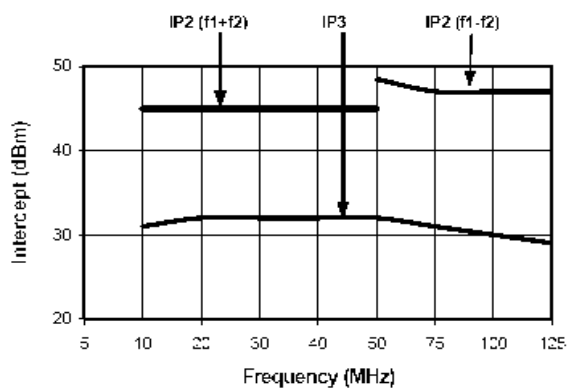
Intermodulation Intercept
