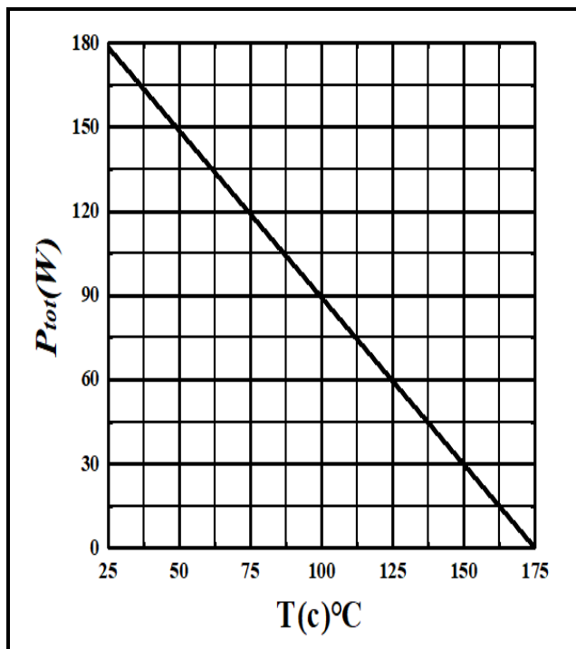
Figure 5. Power derating
