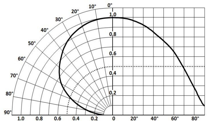
Typical Polar Radiation Plot - B120
