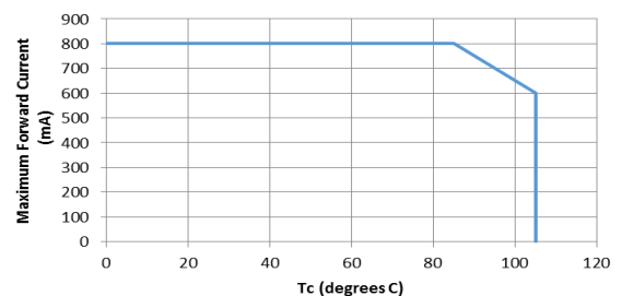
CDM-14 Maximum Forward Current vs. T_c
