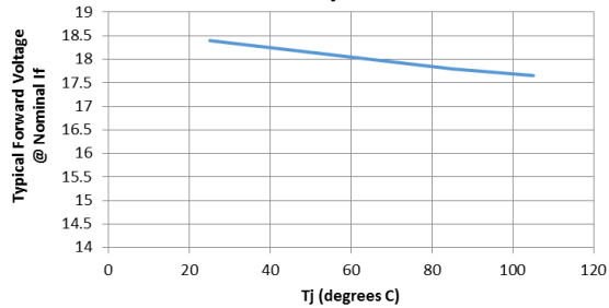
CDM-6 Typical V_f @ Nominal I_f vs. Junction Temperature
